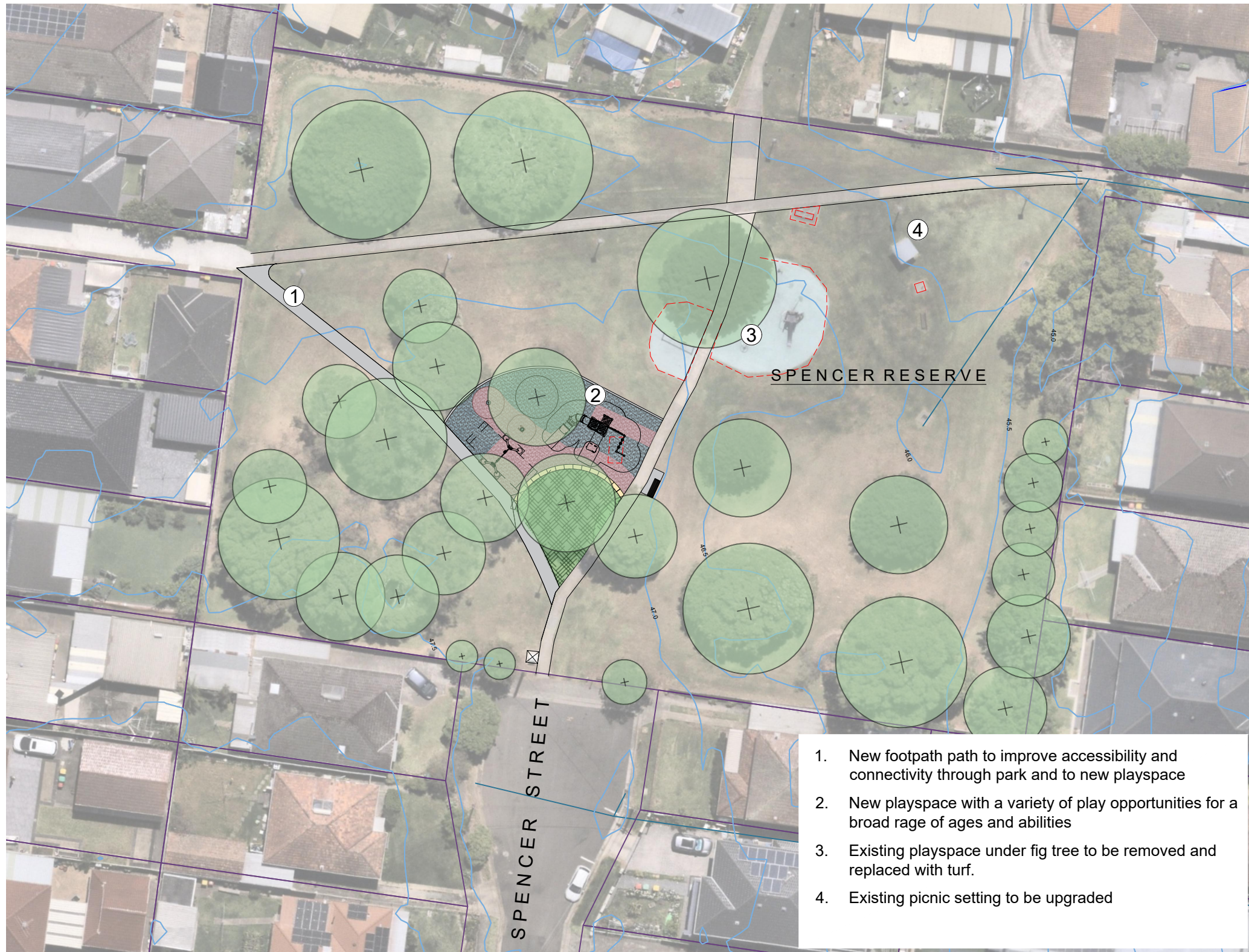
1 Concept Plan Scale 1:500
