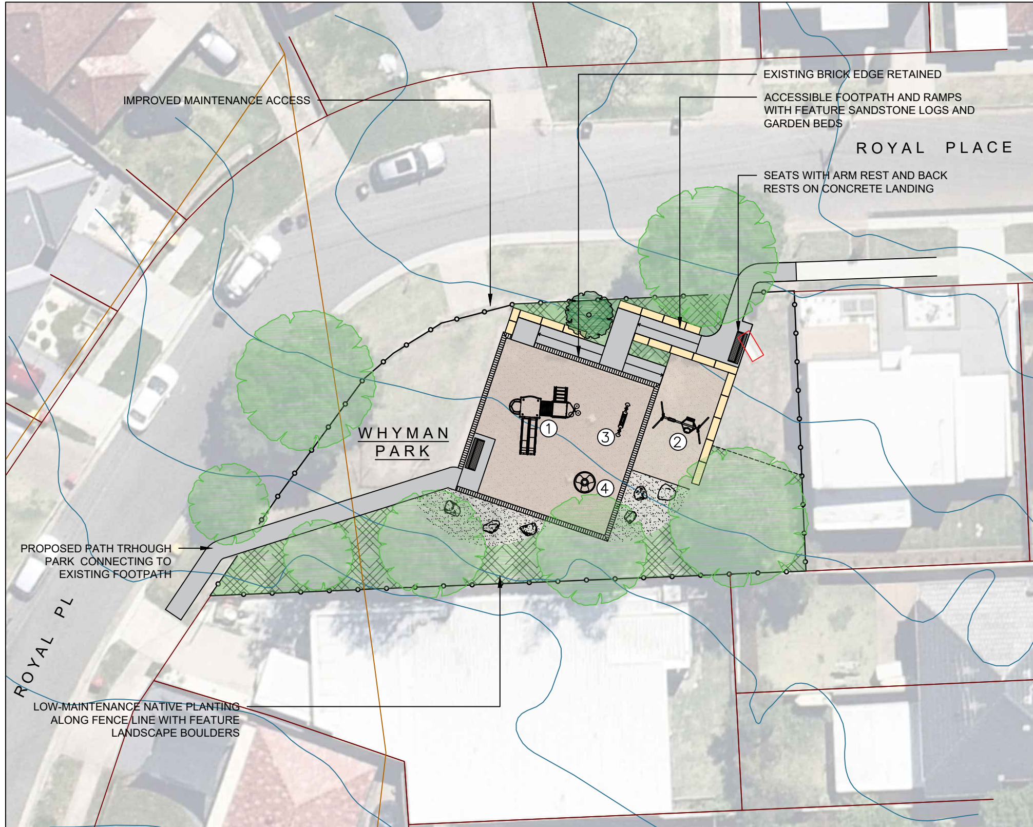
1 Concept Plan Scale 1:250
