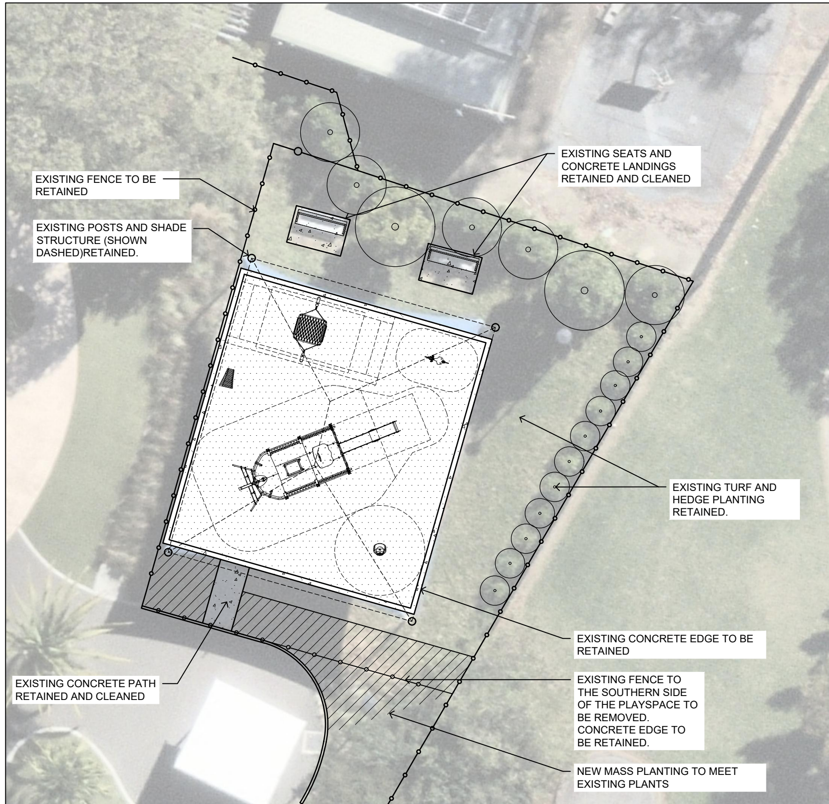
1 Site Plan Scale 1:150 @ A3
