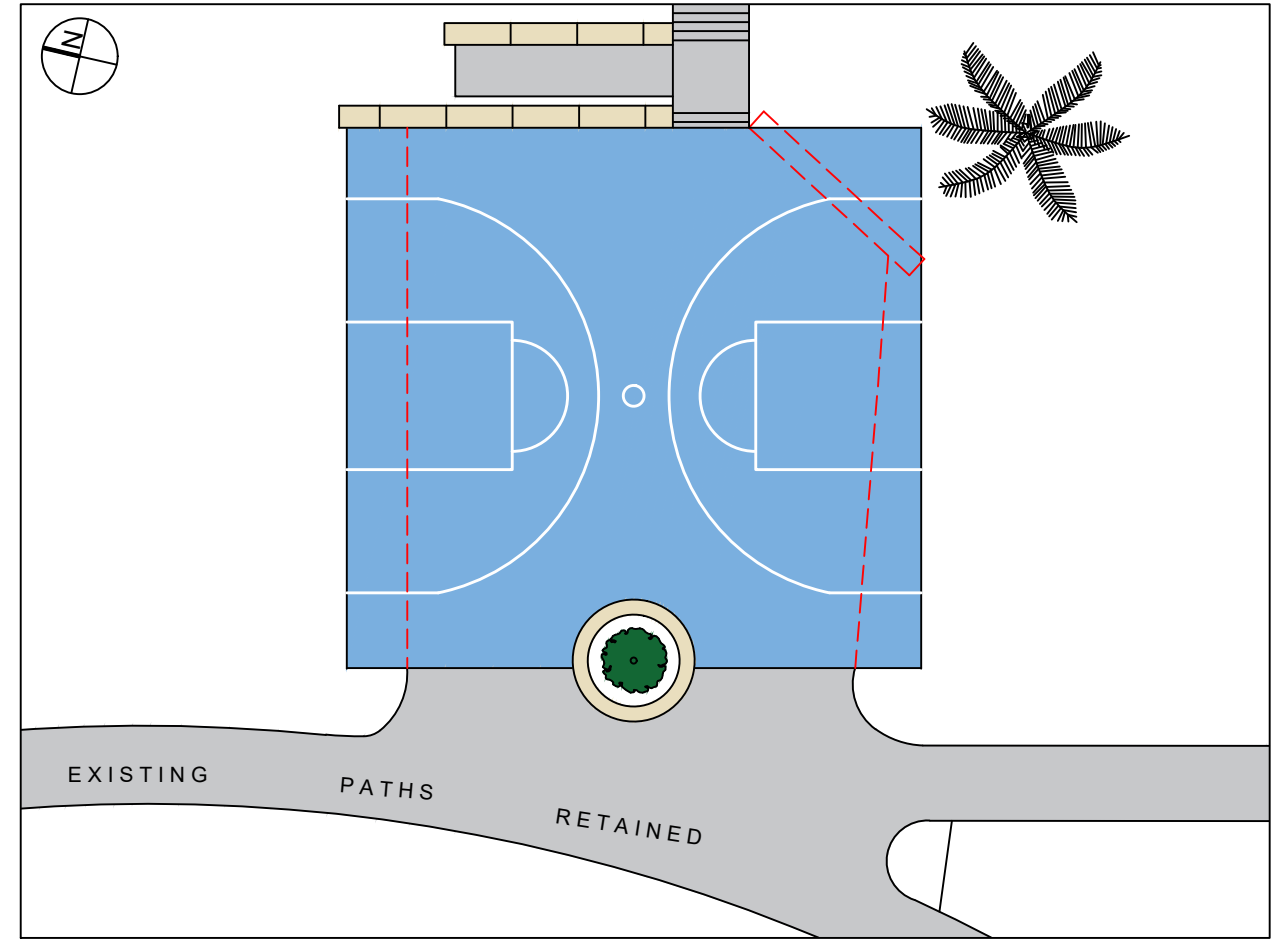
2 Concept Plan Scale 1:250
