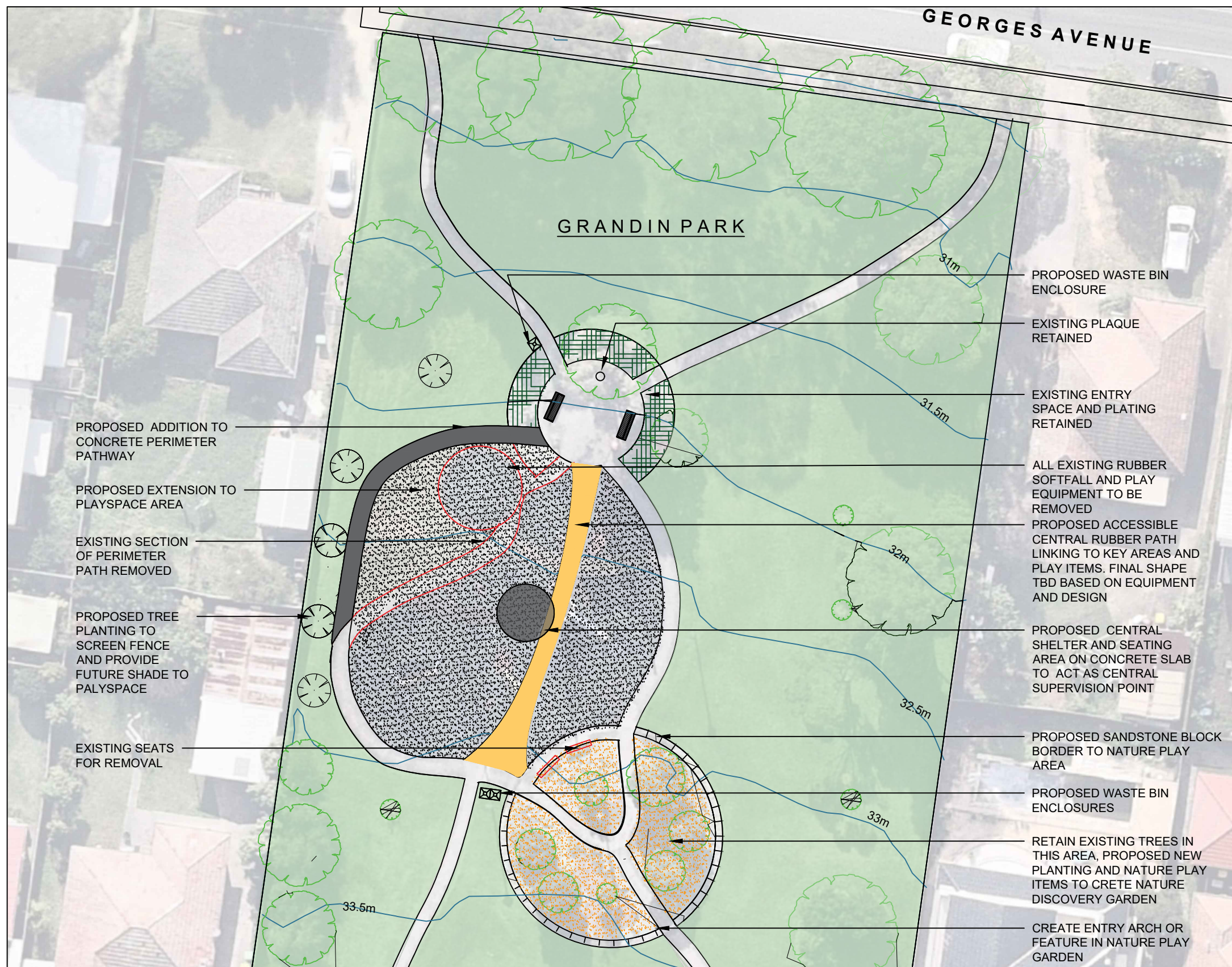
1 Concept Plan Scale 1:300
