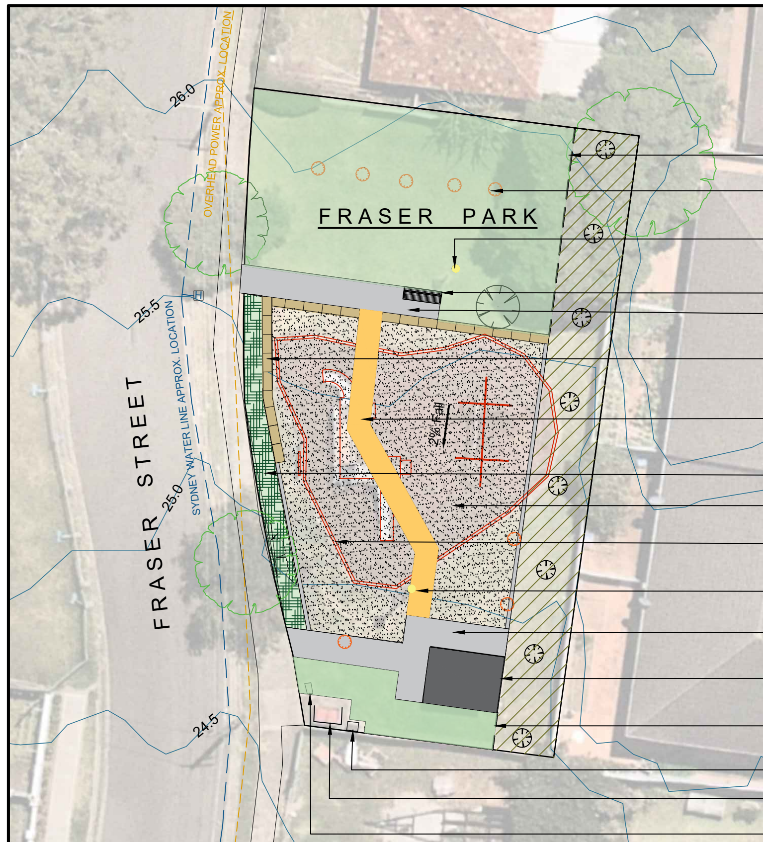
1 Concept Plan Scale 1:200
