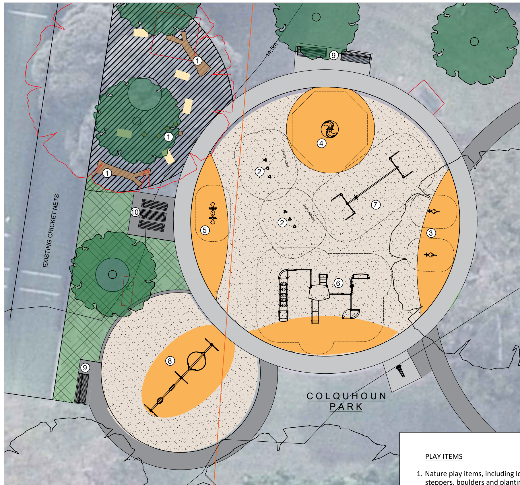
1 Concept Plan Scale 1:150
