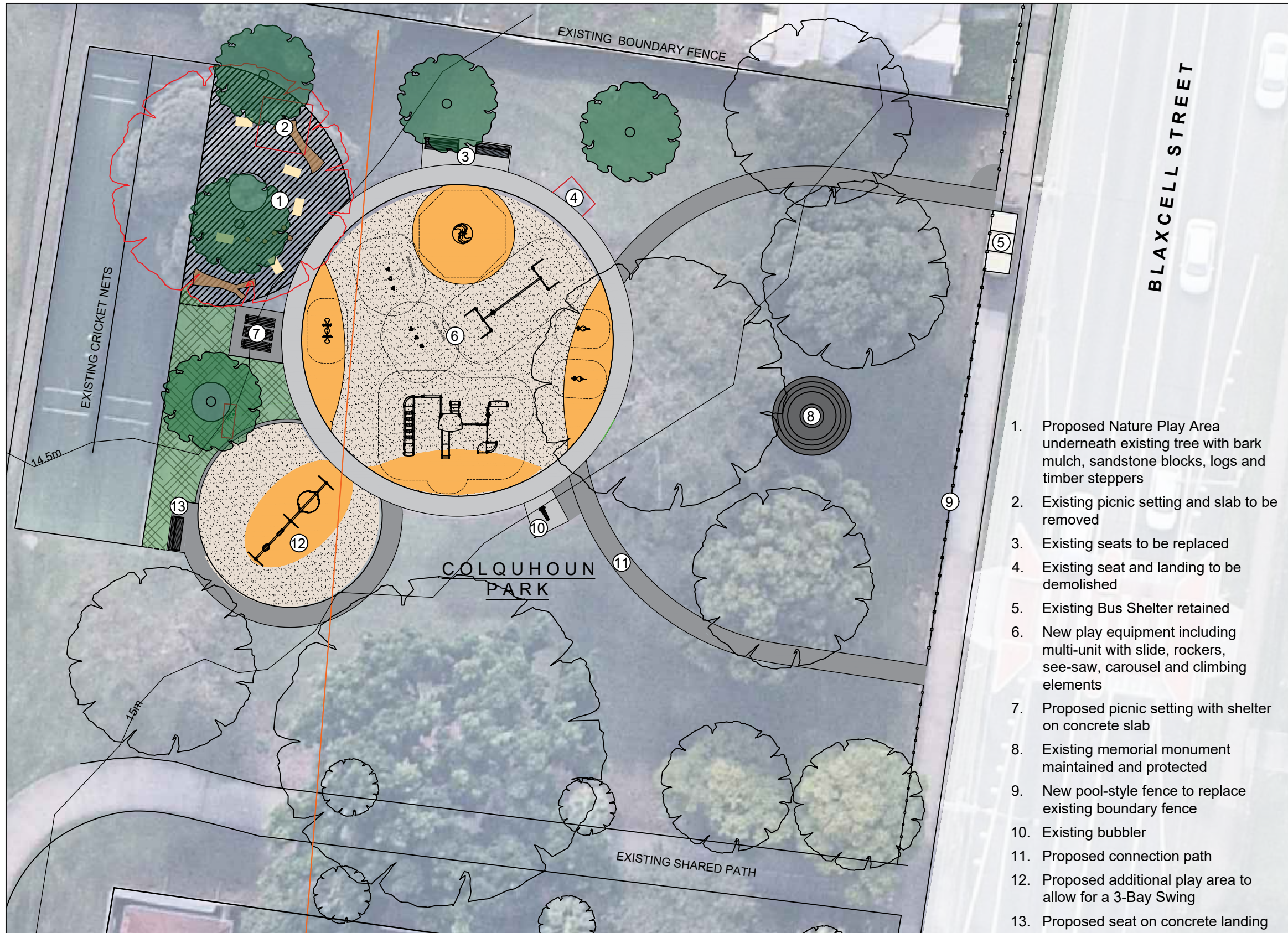
1 Concept Plan Scale 1:250
