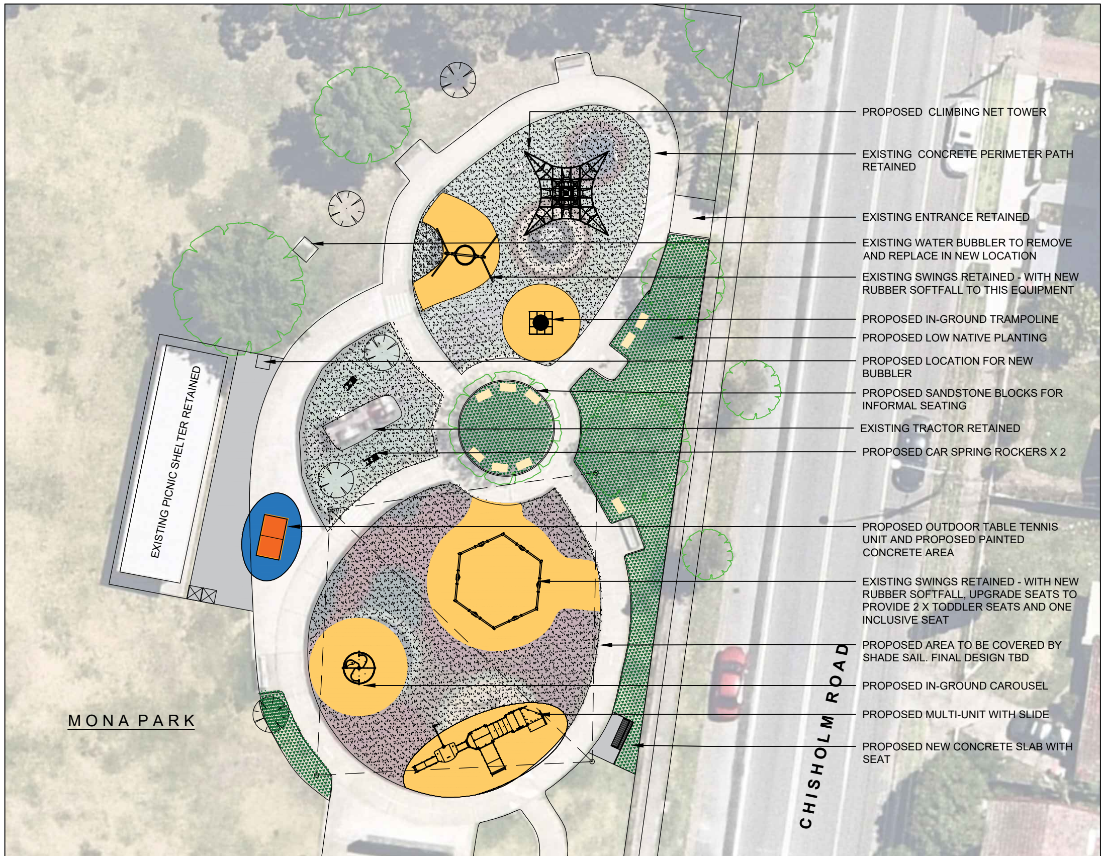
1 Concept Plan Scale 1:250
