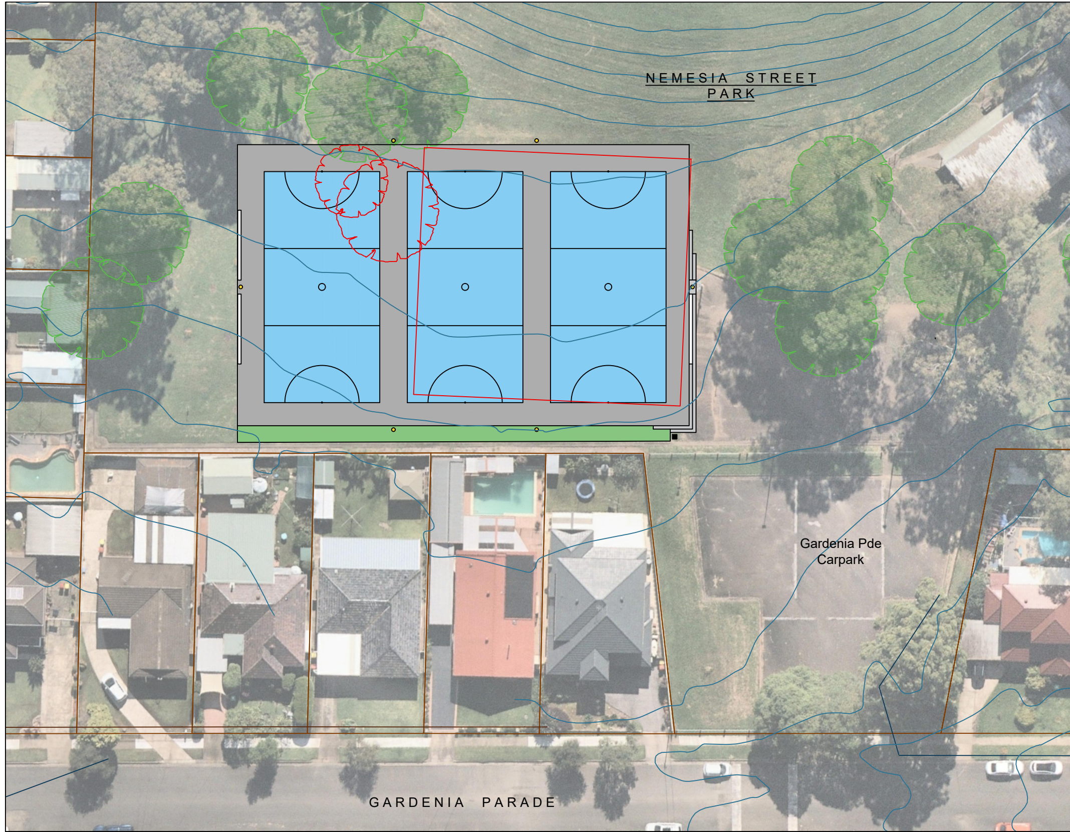
1 Plan - Netball Courts Scale 1:500
