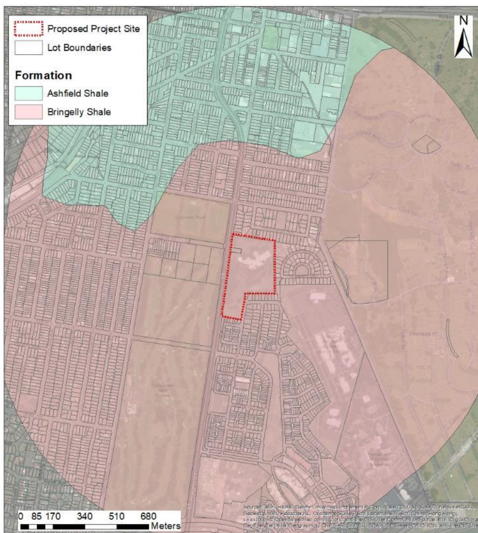
Figure 2-2: Regional geology
