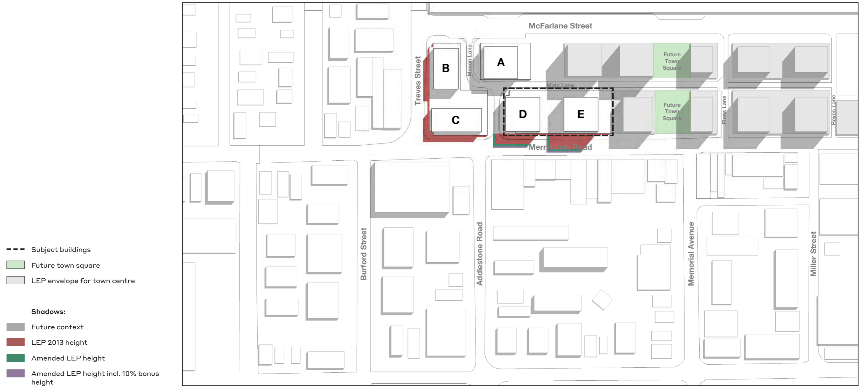
Overshadow Diagram December 21 - 11am (Summer Solstice)
