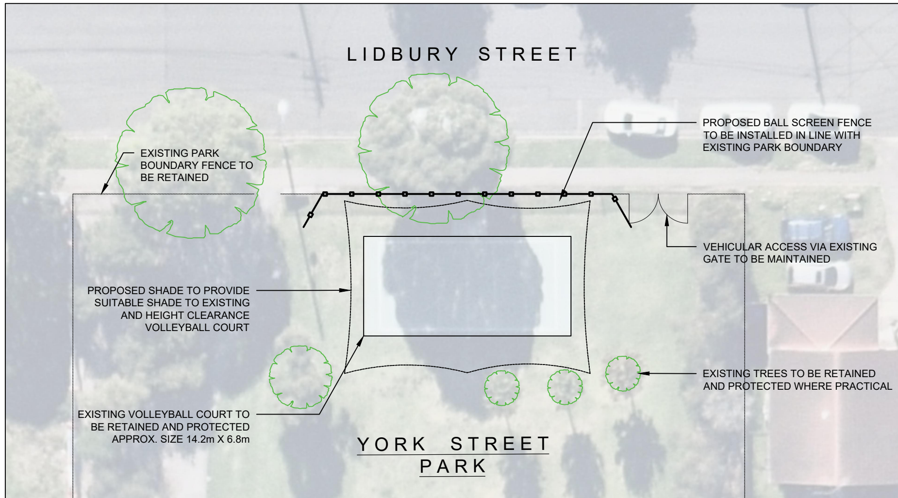
1 Concept Plan Scale 1:250
