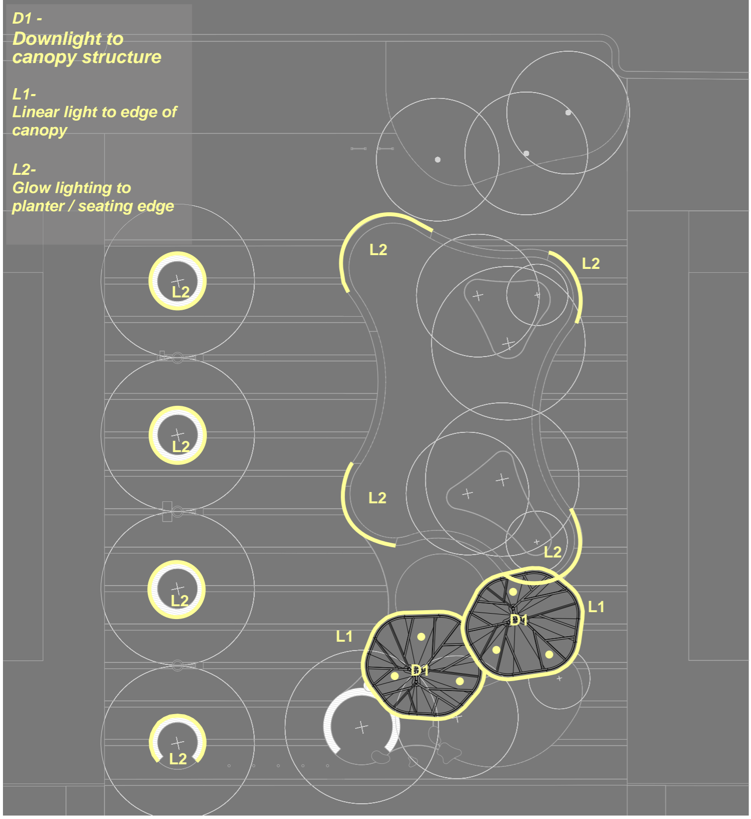
Type D1 Downlight to Canopy
